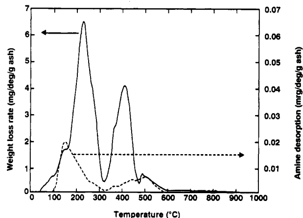
Figure 8. Thermal gravimetric analysis (solid) and temperature programmed amine desorption (dashed) of an as-synthesized MCM-41(40) made using \text{C}_{16}\text{H}_{33}(\text{CH}_3)_3\text{N}^+ and containing 2.8% Al. The heating rate was 20 °C/min.
